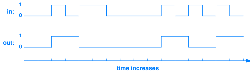
Figure 2.12 Illustration of a transition diagram that shows how a flip flop reacts to the series of inputs in Figure 2.11. Marks along the x-axis indicate times; each corresponds to one bit.
